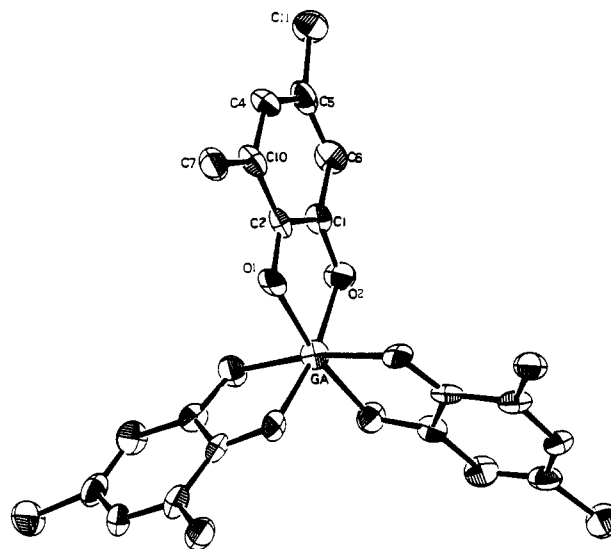
Figure 1. Molecular structure of Ga(TBSQ*) 3 : ORTEP diagram, with atoms drawn as 30% probability ellipsoids. Hydrogen atoms have been omitted for the sake of clarity.
