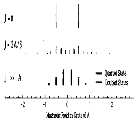
Figure 5. Predicted hyperfine line spectra of a triradical in which each ring has one proton for J = 0 , J = 2A/3 , and J \gg A . In the last case, it is assumed that J \ll kT .
